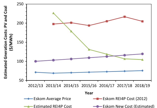
Fig. 10. Cost projections for conventional coal vs. REI4P. Source: Price information has been obtained from own data; NERSA [49]; and U.S. Energy Information Administration [46].
