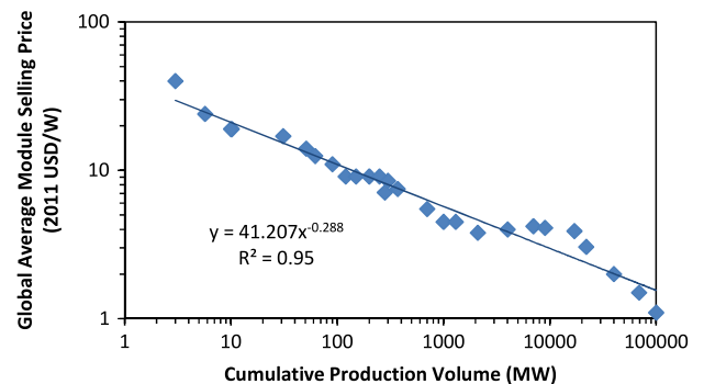
Fig. 2. PV module selling prices decrease with cumulative production. Source: IRENA [47].
