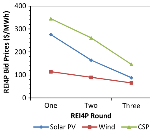
Fig. 9. REI4P bid prices more competitive in the recent rounds.
