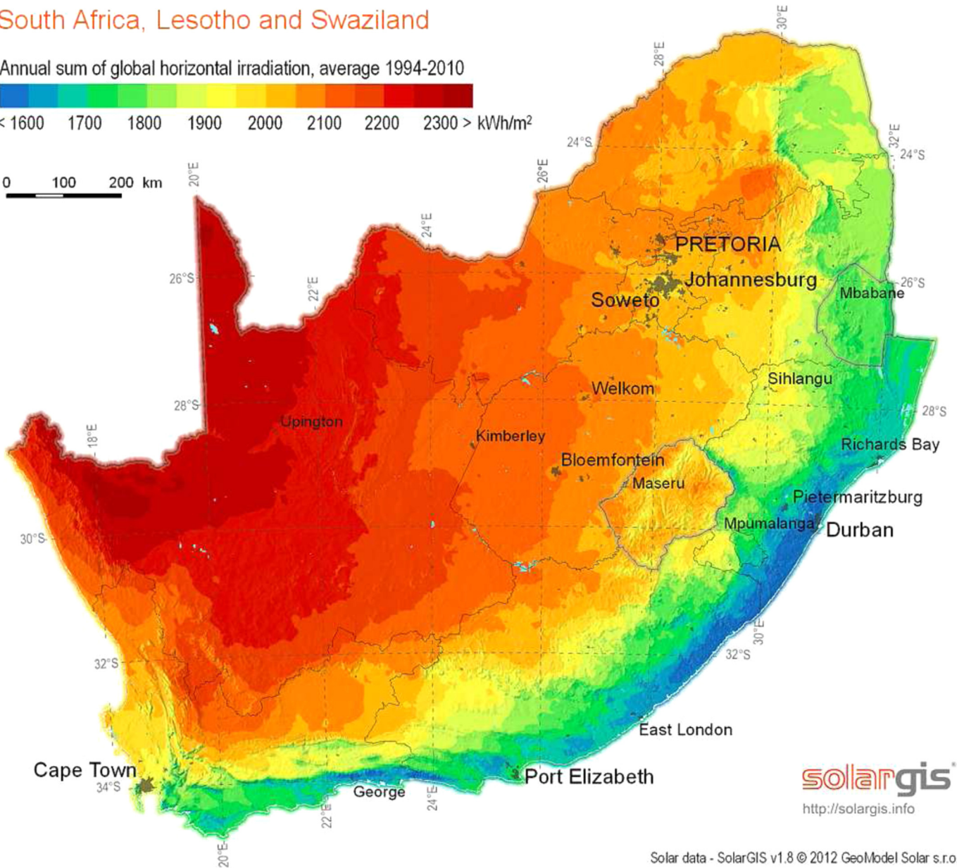
Fig. 4. Solar resource quality across South Africa.
