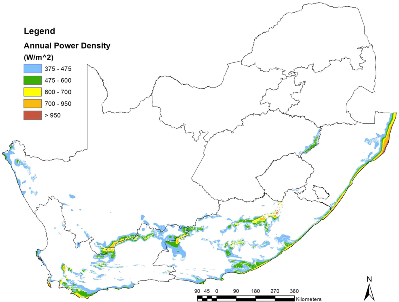
Fig. 3. Best wind resource quality areas in South Africa.
