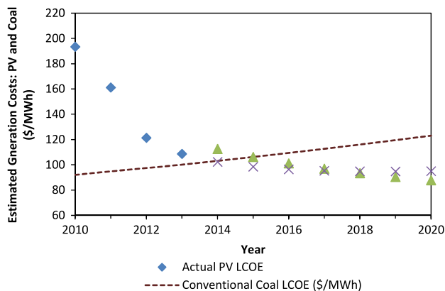
Fig. 8. Actual and predicted LCOE costs for PV power. Source: PVinsights [48] and own calculations.
