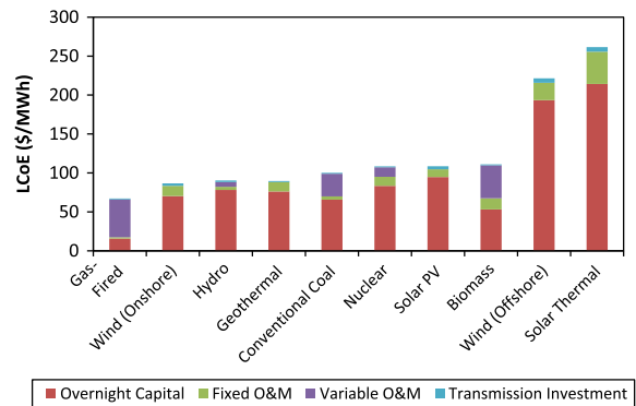
Fig. 1. Total cost of generation by technology. Source: U.S. Energy Information Administration [46].
